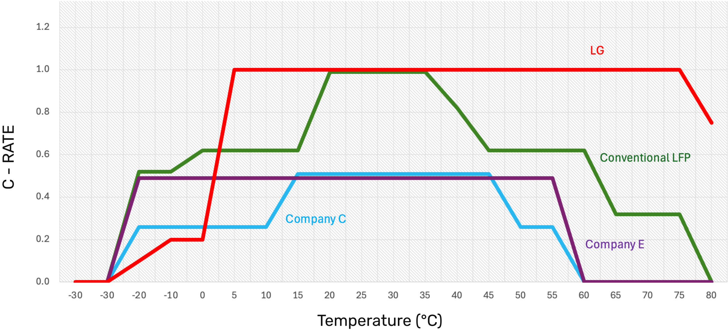
Maximum charge power
